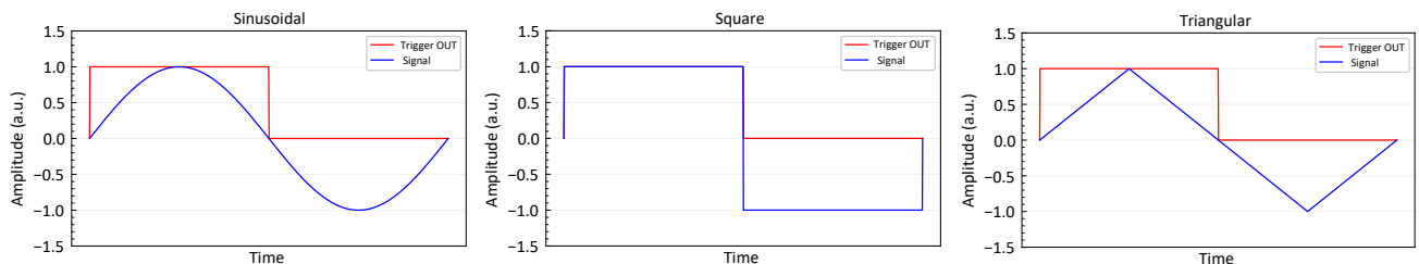
Figure 8: Different waveforms overlapped with the corresponding Trigger OUT signal.
