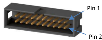
Figure 4: Connector 4 : Würth Electronics header 100 mil 90deg.
